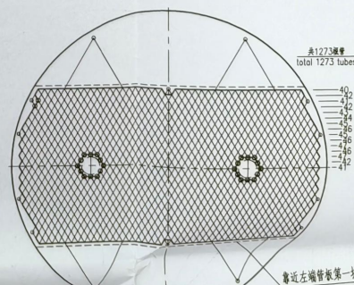
换热管布管详图 Detailed drawing of heat exchange tube layout 1:14
